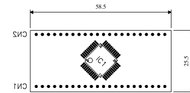
DIP44 PITCH=20.32 ( 800mil )
